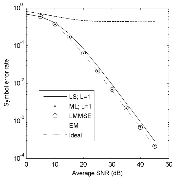
Figure 8 16-QAM SER versus total average SNR \bar{\gamma} for various algorithms. The OFDM system employs two consecutive identical symbol blocks for frequency tracking and channel estimation for the same bandwidth efficiency. \delta = 0.2 . Also included is the ideal system 16-QAM SER with perfect frequency synchronization and channel estimation.
