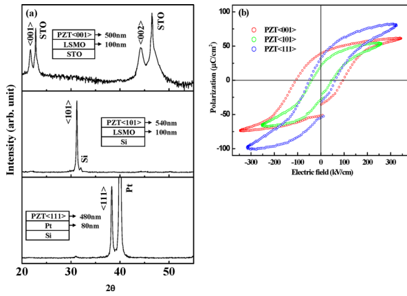
FIG. 1. (Color online) X-ray diffraction pattern of PZT thin films with (a) \langle 001 \rangle , \langle 101 \rangle , and \langle 111 \rangle orientations deposited on LSMO/STO (upper panel), LSMO/Si (middle panel), and Pt/Si (lower panel) substrates, respectively. (b) P - E hysteresis loops of PZTs.
