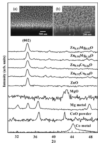
FIG. 1. XRD measurements of the well-aligned Zn_{1-x}Co_xO and Zn_{1-x}Mg_xO nanorods and references MgO, CoO, Co, and Mg metals (on the logarithmic scale). Insets [(a) and (b)] display SEM images of Zn_{1-x}Co_xO ( x=0.08 ) and Zn_{1-x}Mg_xO ( x=0.03 ) nanorods.
