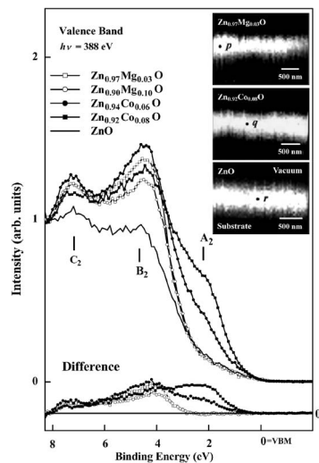
FIG. 4. Valence-band photoemission spectra obtained from selected positions p , q , and r shown in the upper inset, which present the Zn 3 d SPTEM cross-sectional images of the well-aligned Zn 1-x Mg x O ( x =0.03), Zn 1-x Co x O ( x =0.08), and ZnO nanorods. The lower inset shows the difference valence-band spectra of Zn 1-x Co x O and Zn 1-x Mg x O with respect to ZnO nanorods.
