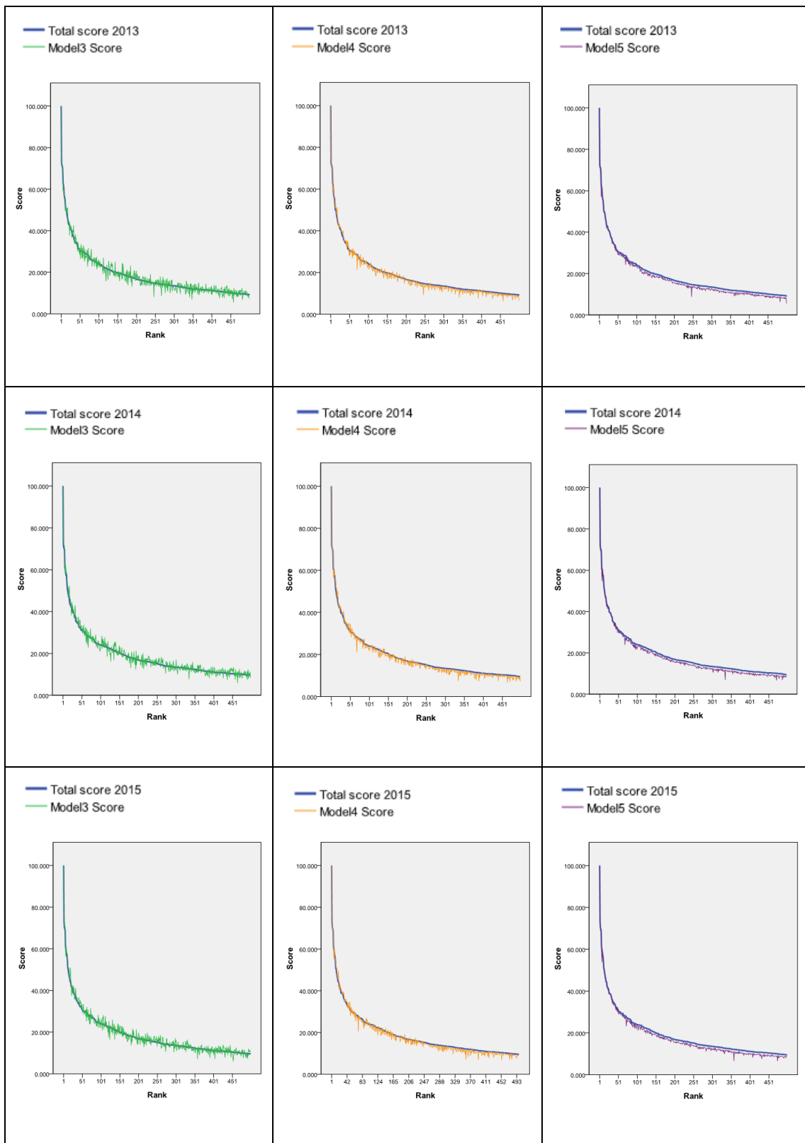
Figure 4. Scores of modified Models 3, 4 and 5 with the actual scores of ranks 1 to 500 from 2013 to 2015
