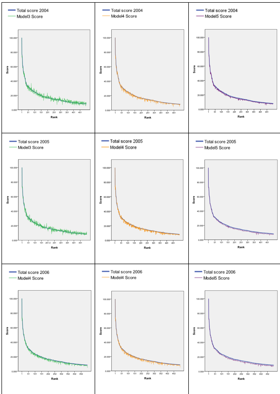
Figure 1. Scores of modified Models 3, 4 and 5 with the actual scores of ranks 1 to 500 from 2004 to 2006
