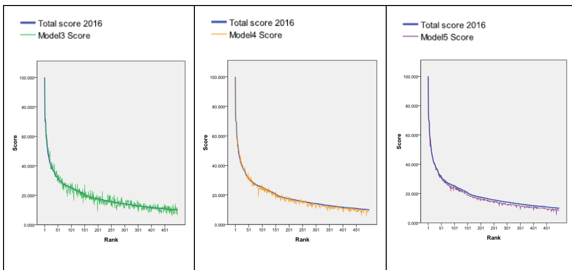
Figure 5. Scores of modified Models 3, 4 and 5 with the actual scores of ranks 1 to 500 in 2016
