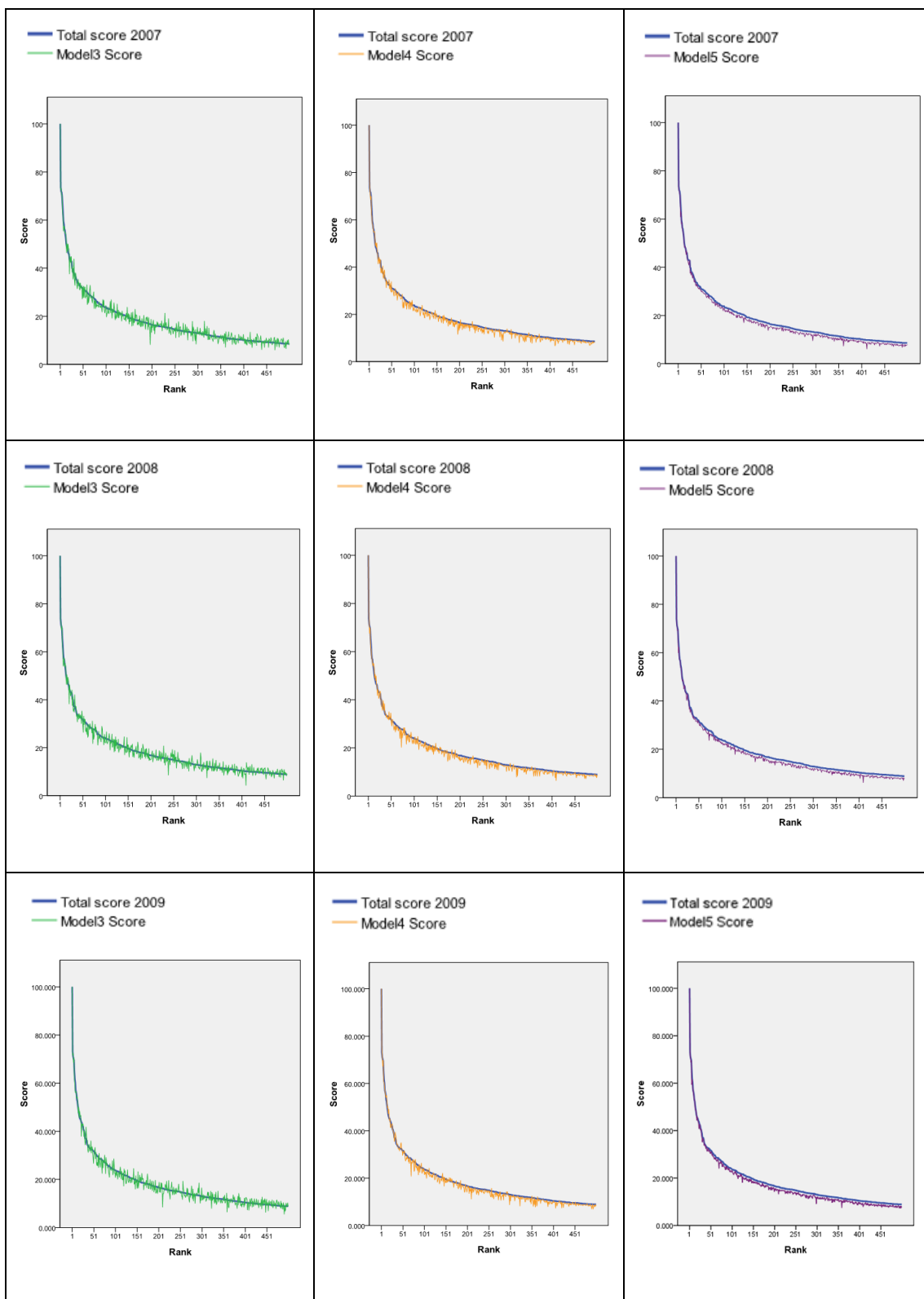
Figure 2. Scores of modified Models 3, 4 and 5 with the actual scores of ranks 1 to 500 from 2007 to 2009
