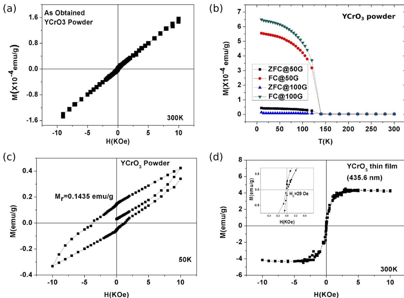
Figure 2 | Magnetization measurements. (a) Paramagnetic behavior of \text{YCrO}_3 powder at room temperature, (b) Temperature dependence of the magnetization for \text{YCrO}_3 powder showing Zero Field Cooled (ZFC) and Field Cooled (FC) curves measured at low fields, and the magnetic transition at 140^\circ\text{K} , (c) the open minor hysteresis loop for the powder at 50\text{ K} upon field cooling from 300\text{ K} in an external field of 2.5\text{ kOe} , and (d) the hysteresis loop for the amorphous thin film ( 435.6\text{ nm} ) at 300\text{ K} showing robust ferromagnetism with magnetic coercivity, H_c \approx 29\text{ Oe} (inset).
