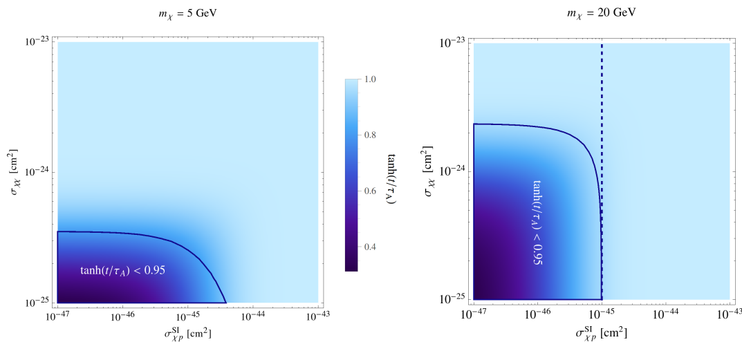
Figure 2. The values of \tanh(t/\tau_A) over \sigma_{\chi p}^{\text{SI}} - \sigma_{\chi\chi} plane at the present day, t = t_{\odot} . The blue-circled area is the non-equilibrium region for N_{\chi} . The vertical line at the right panel indicates the LUX bound, \sigma_{\chi p}^{\text{SI}} \leq 10^{-45} \text{ cm}^2 , for m_{\chi} = 20 \text{ GeV} .
