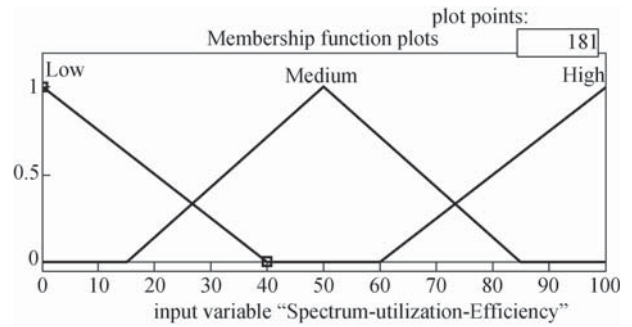
Fig. 9 Membership function of Spectrum utilization Efficiency
