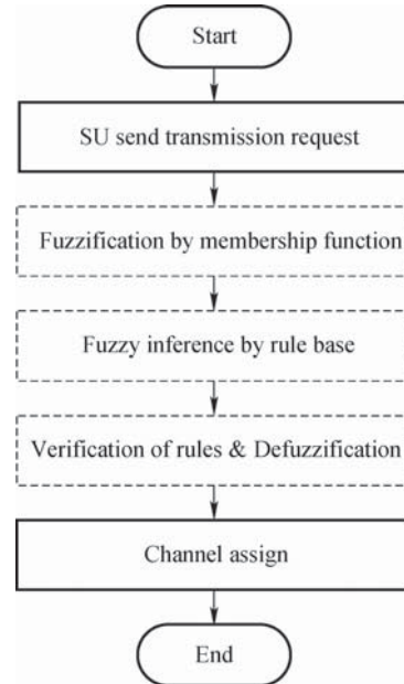
Fig. 7 Flow chart for SU priority scheduling
