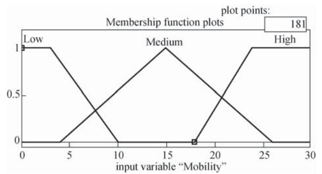
Fig. 10 Membership function of Mobility
