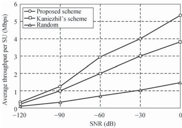
Fig. 14 Analysis of average throughput per SU
