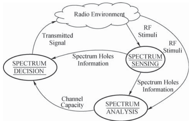
Fig. 2 Cognitive cycle
