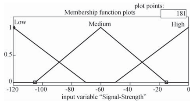
Fig. 12 Membership function of Signal Strength
