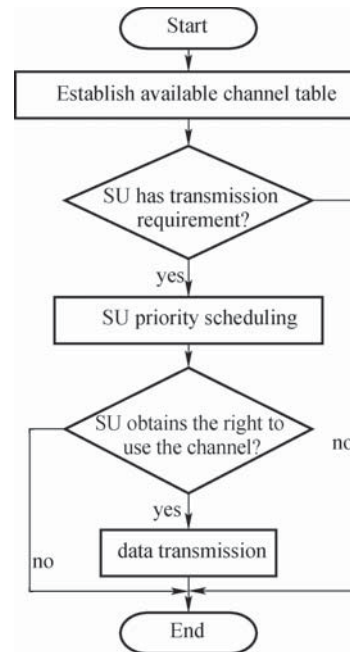
Fig. 4 Fuzzy-based dynamic channel allocation scheme
