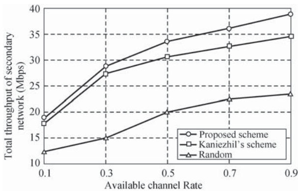
Fig. 15 Analysis of total throughput of secondary network
