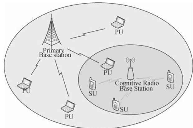
Fig. 5 System model
