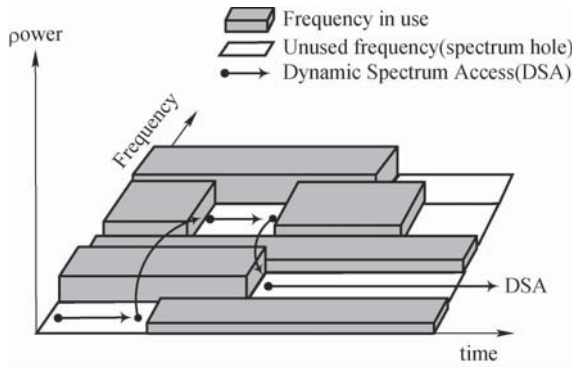
Fig. 1 Dynamic spectrum access (DSA)
