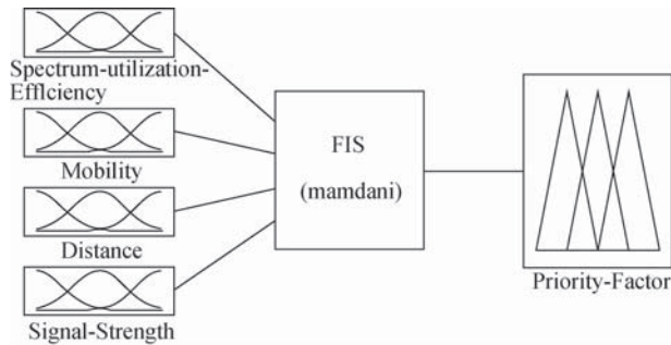
Fig. 8 Model of the proposed FIS
