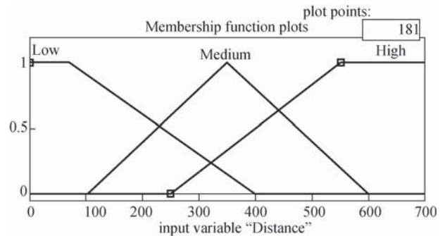
Fig. 11 Membership function of Distance
