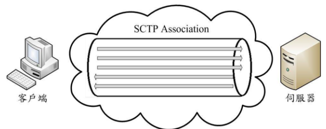
圖二、Multi-Streaming概念圖
