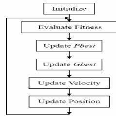
Figure. 4 PSO calculation Process
