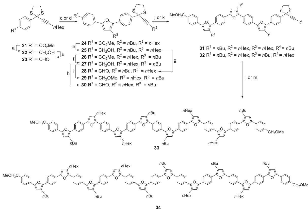
Scheme 4. Formation of alternating benzene–furan oligomers with different substituent groups. a) DIBAL, 98 %; b) \text{MnO}_2 , 92 %; c) 1) 21 , n\text{BuLi} , -78^\circ\text{C} , 2) 5 , 3) TFA; yield of 24 = 53 %; d) 1) 6 , 2) TFA; yield of 26 = 50 %; e) DIBAL; yield of 25 = 93 %; f) DIBAL; yield of 27 = 90 %; g) \text{MnO}_2 ; yield of 28 = 91 %; h) \text{MnO}_2 ; yield of 30 = 90 %; i) \text{NaH}/\text{MeI} ; yield of 29 = 93 %; j) 1) 29 , n\text{BuLi} (1.1 equiv), 2) 28 , 3) TFA; yield of 31 = 49 %; k) 1) 29 , n\text{BuLi} (1.1 equiv), 2) 30 , 3) TFA; yield of 32 = 68 %; l) 31 , n\text{BuLi} (1.1 equiv), 2) terephthalaldehyde, 3) TFA; yield of 33 = 45 %; m) 32 , n\text{BuLi} (1.1 equiv), 2) 5 , 3) TFA; yield of 34 = 66 %.
