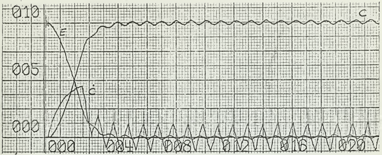
plant output, velocity and error vs. time
