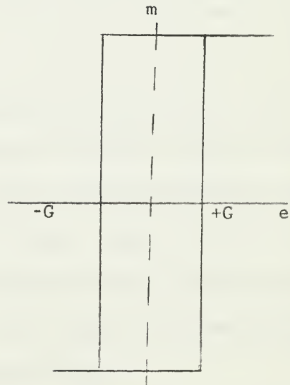
Fig. 2-8 Two-position control with differential gap
