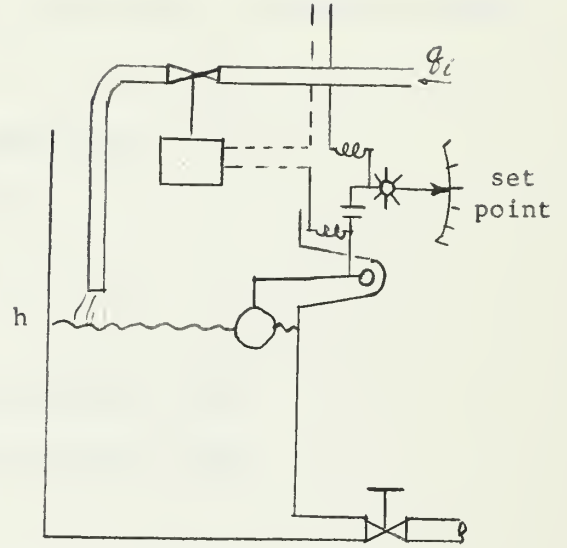
Fig. 2-6. Two position control
