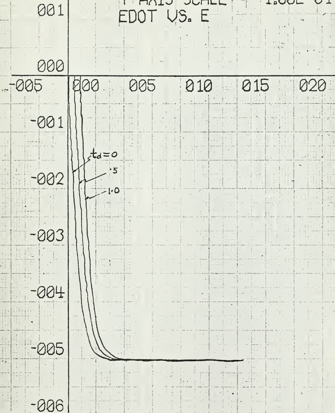
Fig. 10-2. Phase trajectory of relay servo system, relay voltage .5 volt
