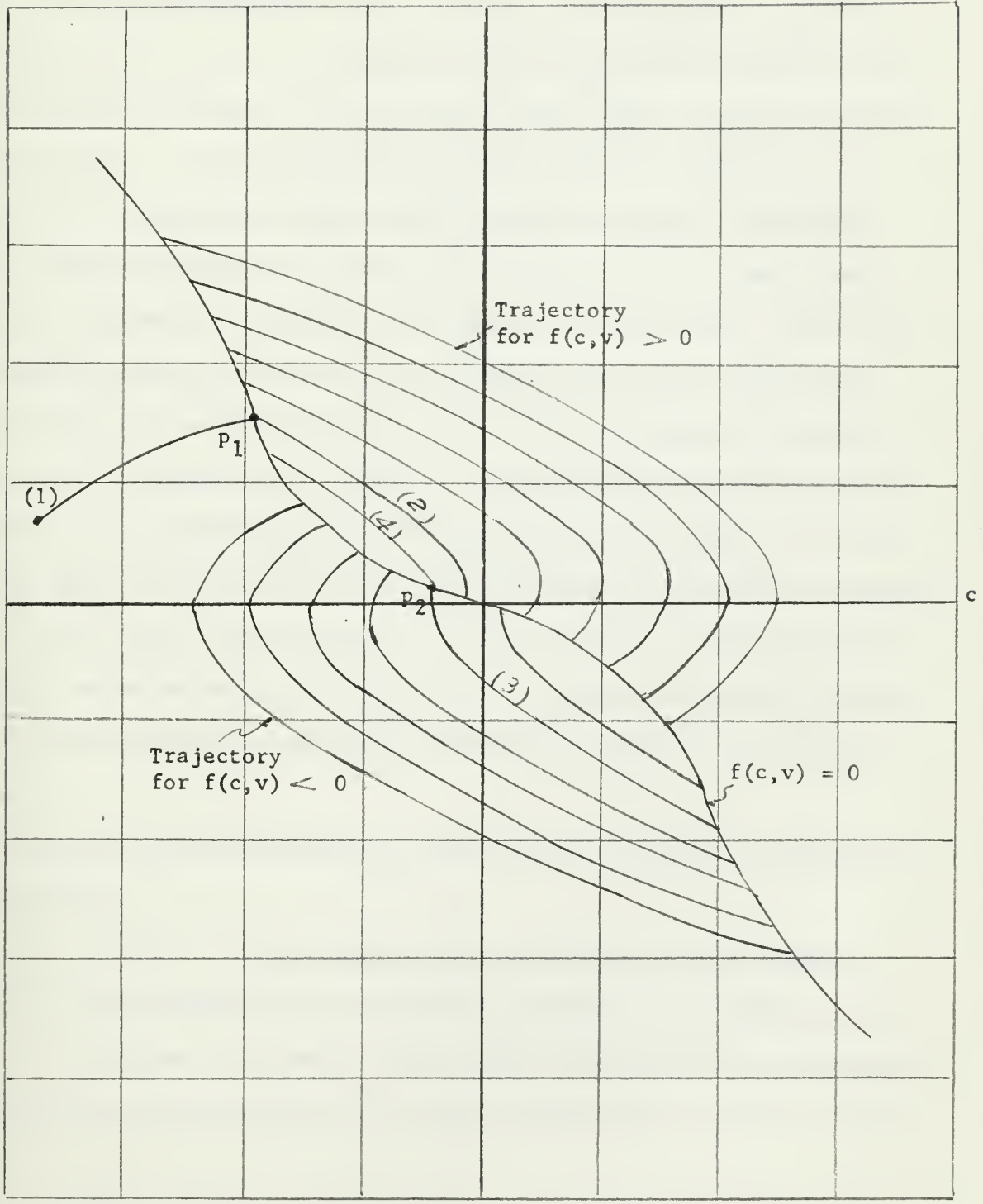
Fig. 2-3. Switching line for contactor servomechanism.
