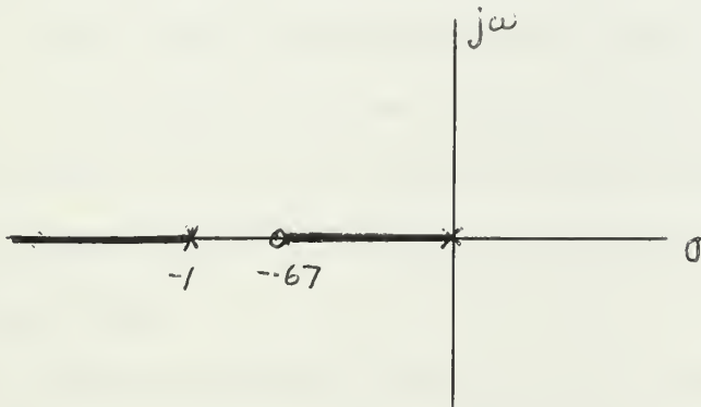
Fig. 8.2. Root locus of Eq. 8.4.
