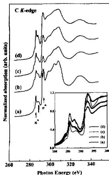
FIG. 2. Normalized C K -edge absorption spectra of (a) the graphite and the CNT with diameters of (b) 220 \pm 100 nm, (c) 30 \pm 15 nm, and (d) 10 \pm 5 nm. The inset displays the enlarged part of the near-edge in a magnified scale.
