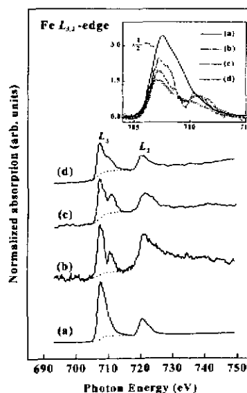
FIG. 3. Normalized Fe L_{3,2} -edge absorption spectra of (a) the Fe metal and the CNTs with diameters of (b) 220 \pm 100 nm, (c) 30 \pm 15 nm, and (d) 10 \pm 5 nm. The dashed line represents the extrapolated background at the Fe L_3 -edge. The center of the continuum step of the arctangent function was selected at the maximum height of the white-line features. The white-line region of the Fe L_3 -edge is shown in the inset in a magnified scale.
