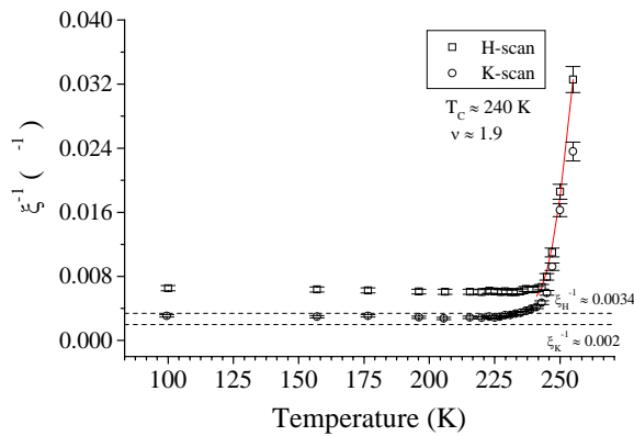
Figure 2: The evolution of correlation lengths along the H and K-direction. The dotted lines are the resolutions along the H and K directions respectively. It is clear to see that the charge stripes do not form a long range ordered state at low temperature, and the red line is the fit of a power law which gives a unusual high exponent \nu \sim 1.9 . This behaviour suggests a quenched disordered charge stripes.
