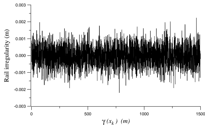
Figure 3: Rail irregularity.
